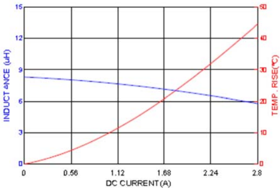
HNR6020NF-8R2
