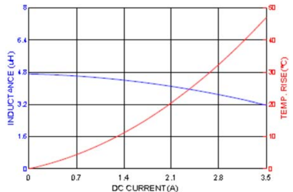
HNR6020NF-4R7
