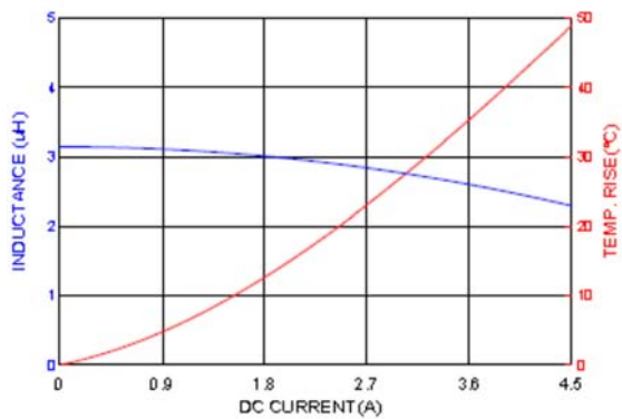
HNR6020NF-3R3
