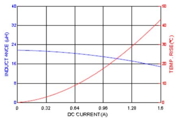
HNR6020NF-220
